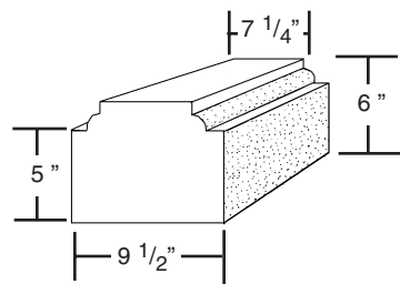
Bottom Rail
