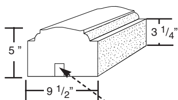
Top Rail
